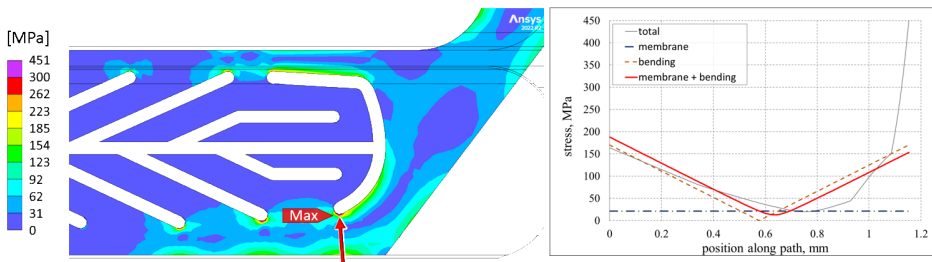
Figure II.8: left side: path for stress linearization at maximum local stress (linear elastic); right side: result of the stress linearization: membrane + bending stress is slightly above the yield stress: 188 MPa
